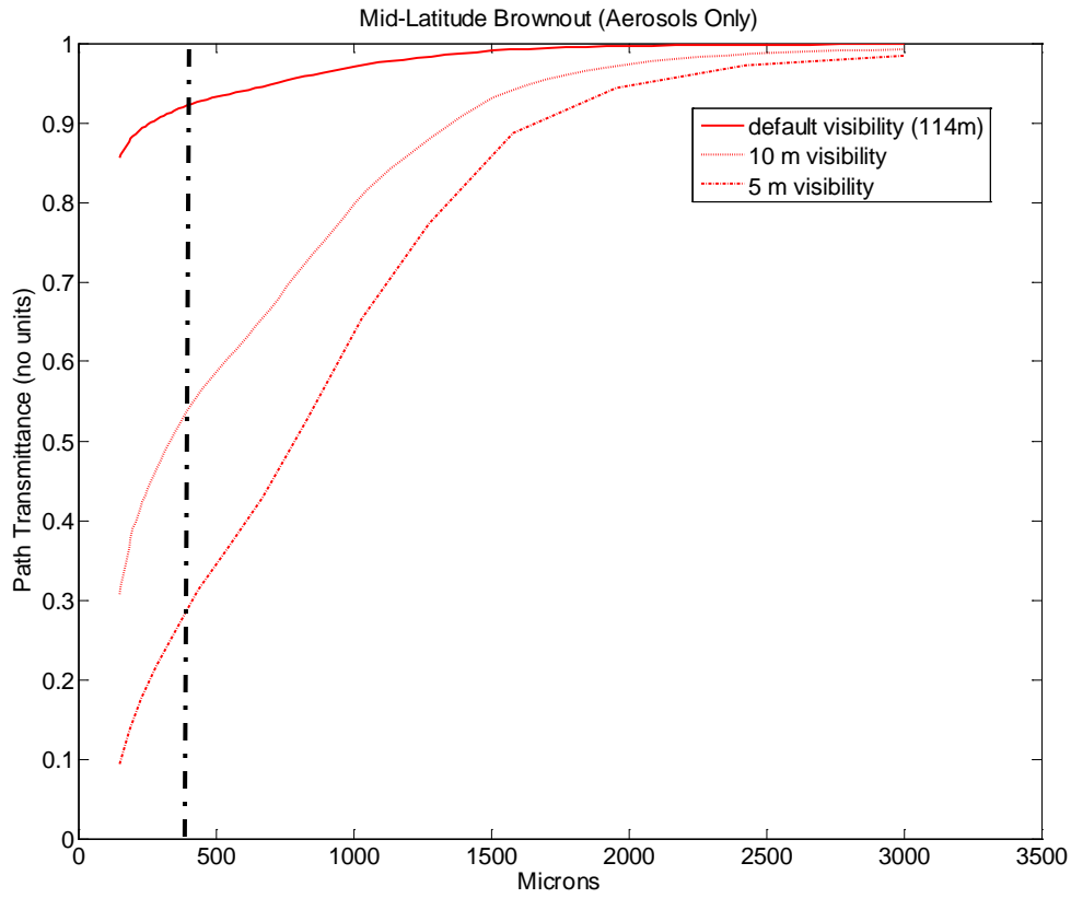
Figure 13. Mid-Latitude brownout aerosol only model transmission across wavelengths from 150μm to 3000μm. The geometry consists of a 15 m propagation path and again molecular effects are not shown, to show the possibility of transmission through different visibilities.
